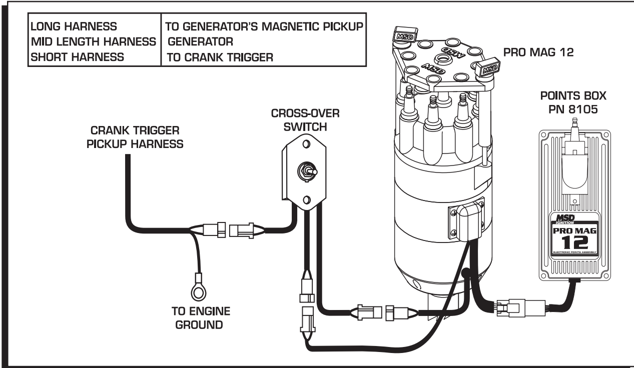
Figure 2 - Wiring the Cross-Over Switch.
