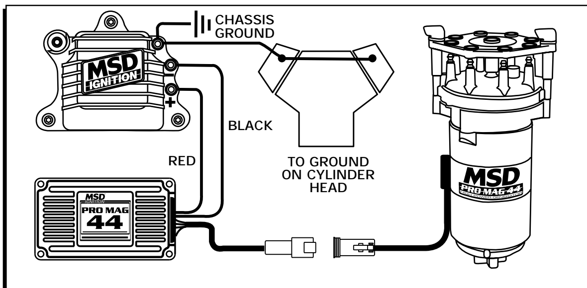
Figure 1 Wiring the Pro Mag 44 Electronic Points Box.
