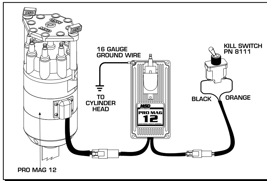
Figure 2 Wiring the 12 Amp Pro Mag.
