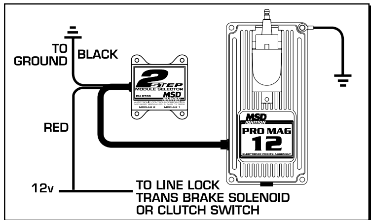
Figure 6 Wiring a Two Step.
