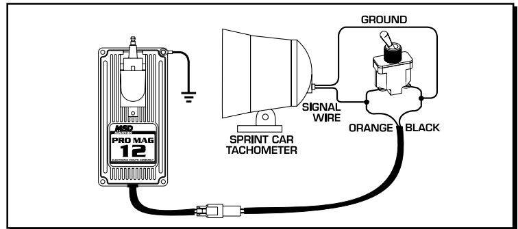
Figure 5 Wiring a Two Step.
