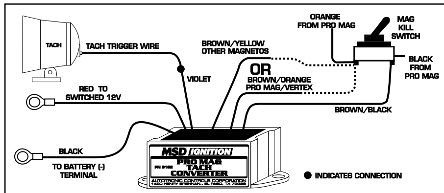
Figure 3 Wiring a Tachometer with PN 8132.
