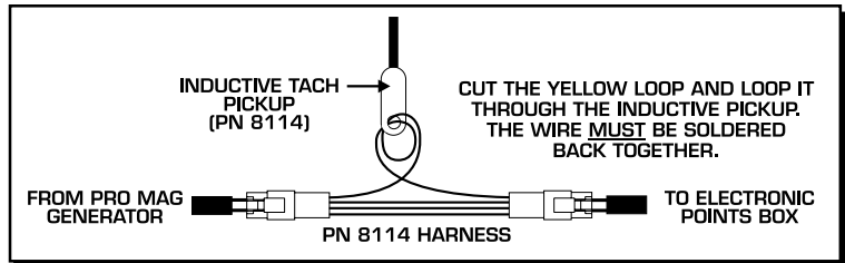
Figure 4 Wiring an Inductive Triggered Tach.
