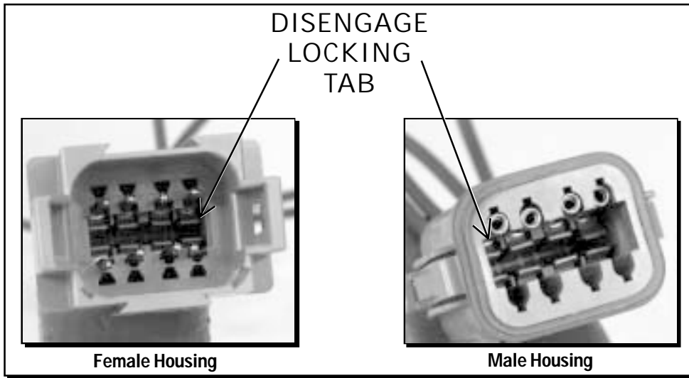
Figure 9 Disassembling the Housings.
