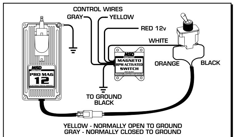
Figure 7 Wiring an RPM Activated Switch.
